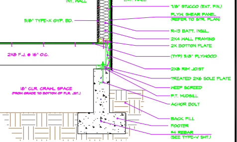
(TYP) FLOOR @ FOUNDATION CONN.
