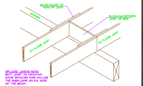
SPLICED JOIST CONN. @ GIRDER
