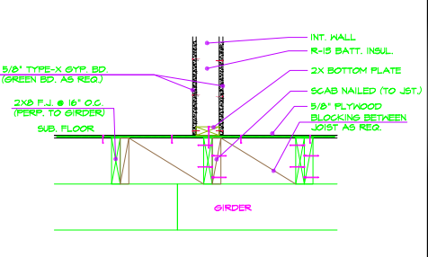
FLOOR @ INT. WALL CONN.
