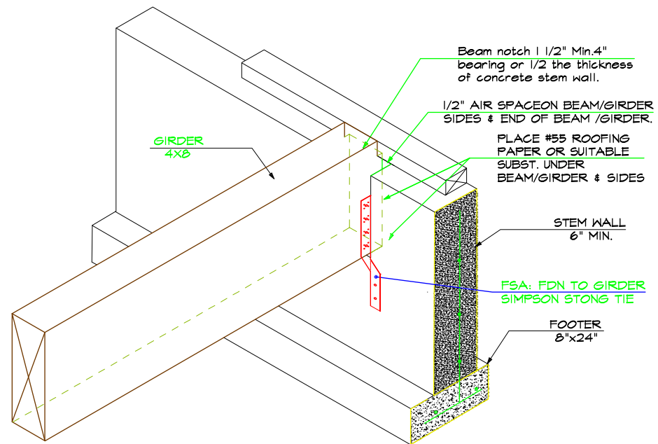
CONC. NOTCH GIRDER SEAT
