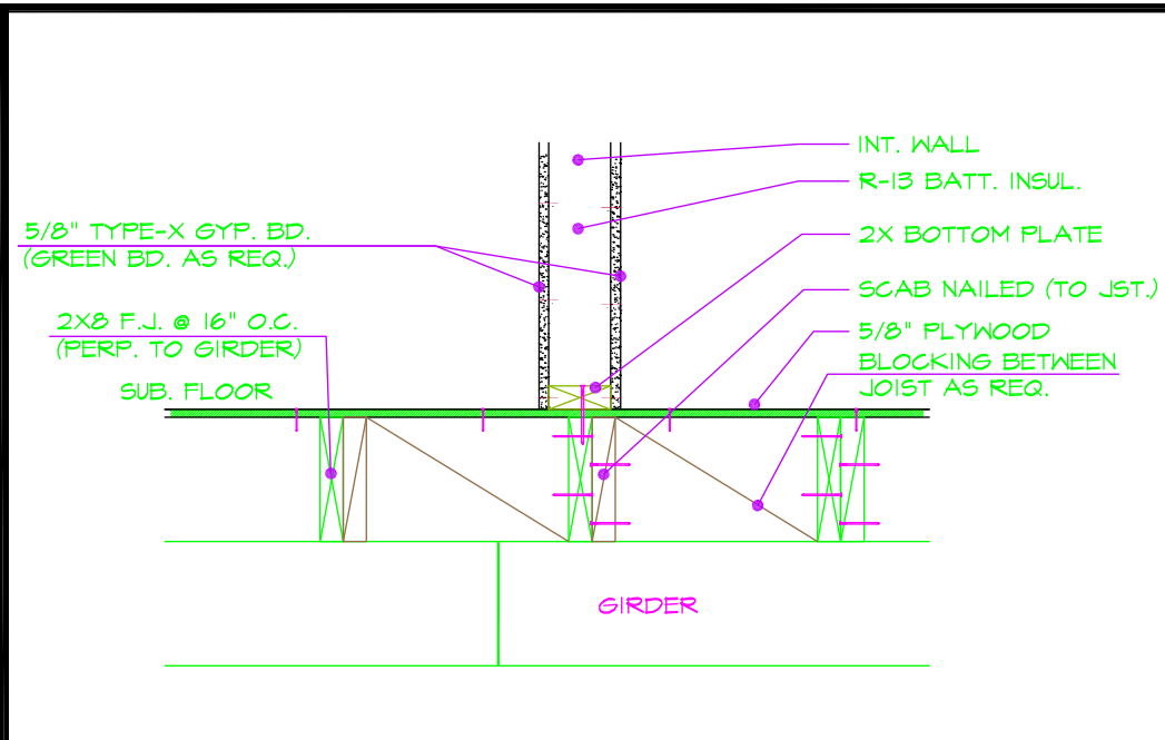
FLOOR @ INT. WALL CONN.
