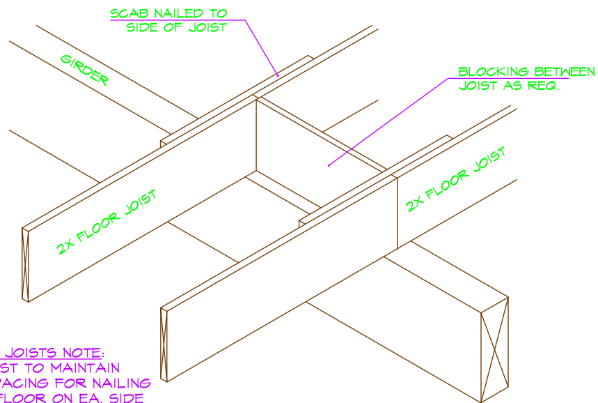
SPLICED JOIST CONN. @ GIRDER
