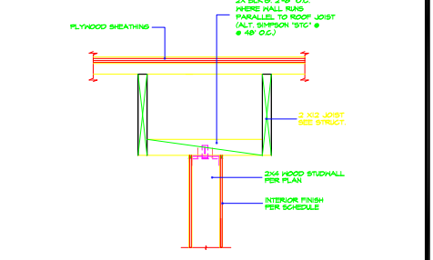
WALL PARALLEL TO JOIST
