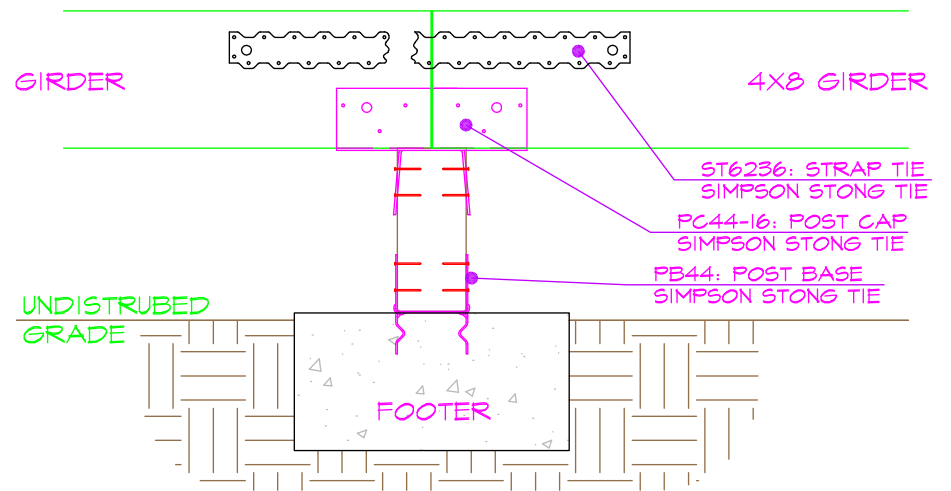
GIRDER/POST CONN. @ FOOTER
