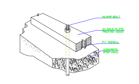
SOLE PLATE @ FOUNDATION
