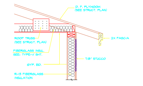
ROOF @ EAVE
