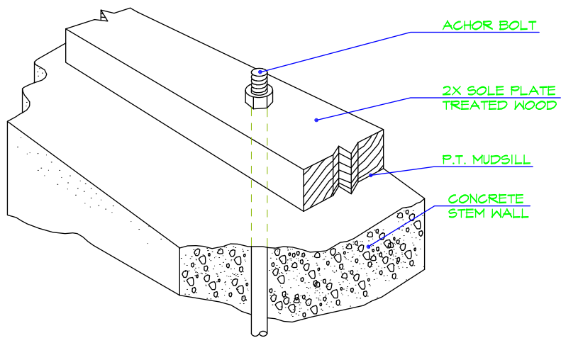
SOLE PLATE @ FOUNDATION
