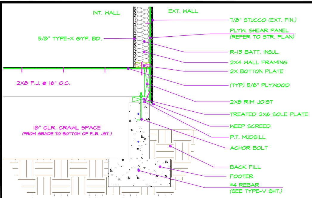
(TYP) FLOOR @ FOUNDATION CONN.
