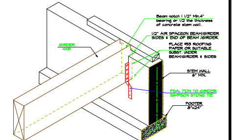
CONC. NOTCH GIRDER SEAT
