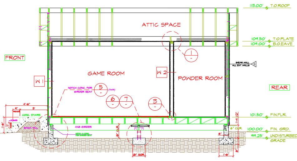
BUILDING SECTION B-B
