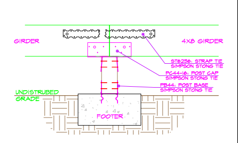
GIRDER/POST CONN. @ FOOTER
